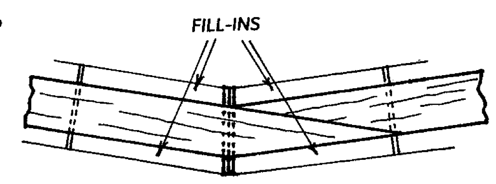
CENTER DIHEDRAL SPLICE
