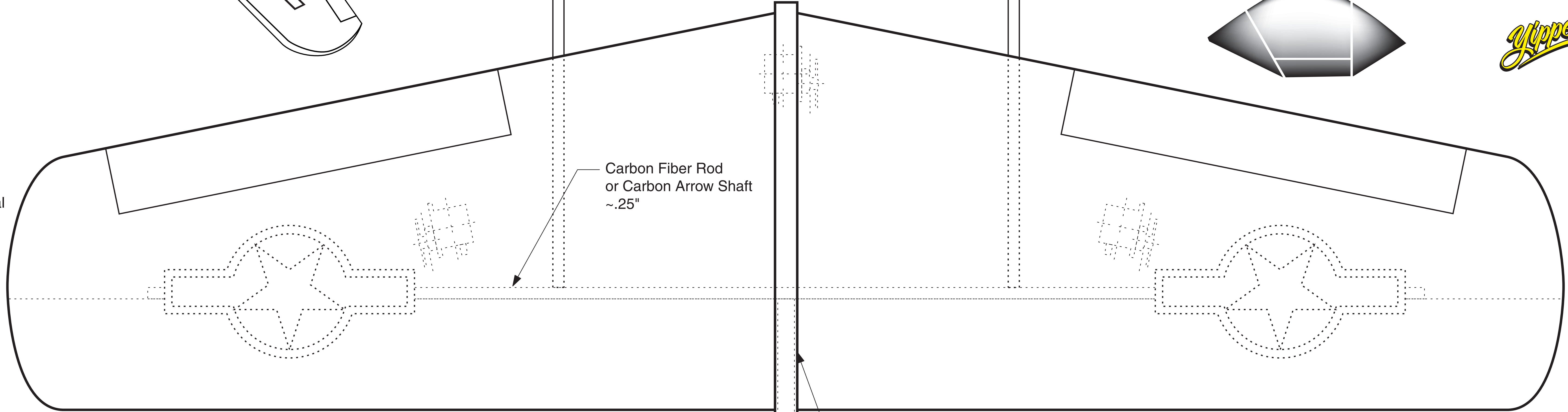
Optional Kline-Fogelman Airfoil Double foam thickness
